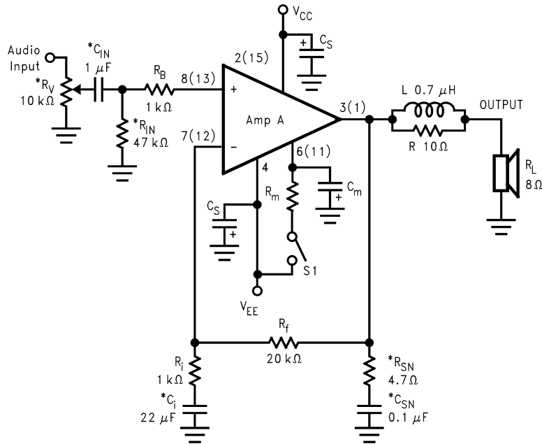
FIGURE 4. Special Audio Amplifier Application Circuit
