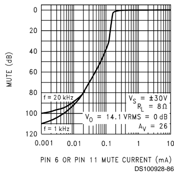
Mute Attenuation vs Mute Current (per Amplifier)
