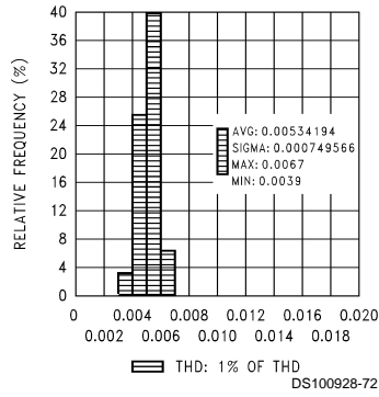
THD+N vs Distribution
