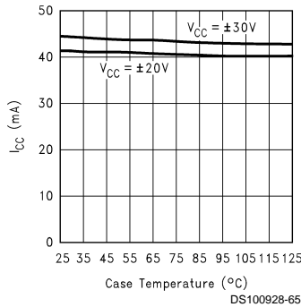
Supply Current vs Case Temperature
