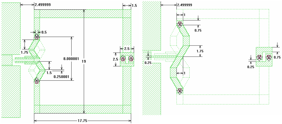
Fig. 2.4b. 915-868 MHz dual band cross tapped loop antenna, "big" type: top layer and bottom layer (top view) (dimensions in mm).
